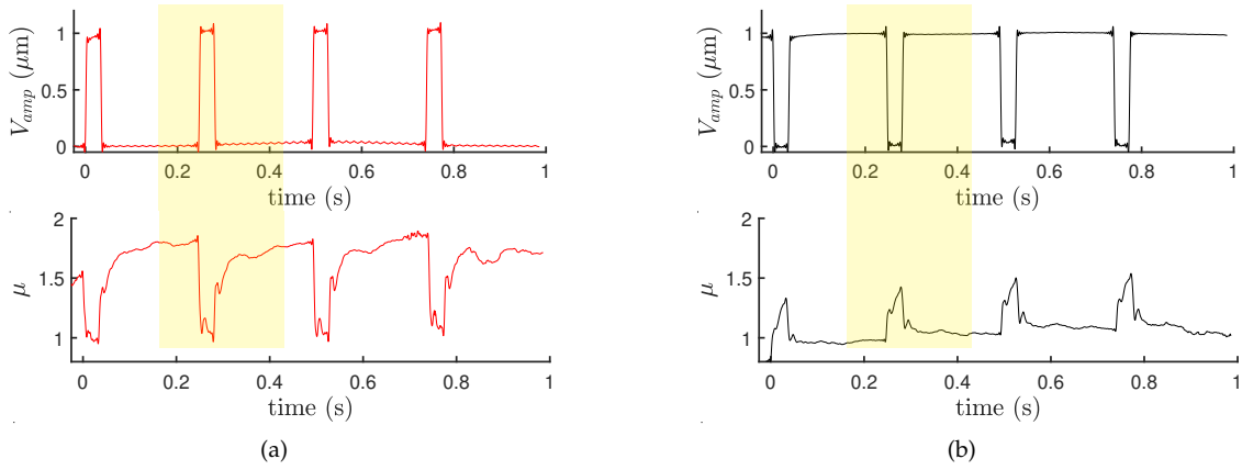
Fig. 10: Vibration amplitude and friction coefficient recorded at 30 mm/s for a) W_{frm}^1 and b) W_{frm}^2 .
