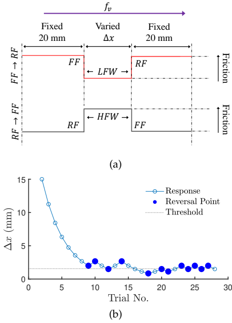
Fig. 3: Experimental procedure for evaluating the spatial threshold distance between two consecutive virtual edges (EXP-1); (a) desired edge sequences ( E_{seq} ), (b) an example for experimental trial.
