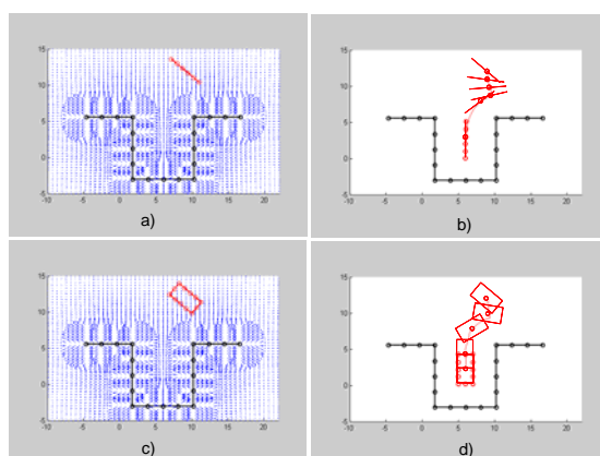
Figure 4. Graphical comparison of the proposed rigid docking approach with the conventional rigid body solution in 2D. A line segment and a rectangular box, made of carbon atoms are separately guided into an artificially created potential well (see the windows a and c respectively). The paths calculated using our approach and the conventional rigid body simulations perfectly overlap with each other for both objects (see the windows b and d).
