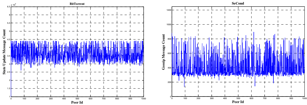
Figure 21. Messages sent: (a) state updates by BitTorrent peers, (b) gossips by SeCond peers
