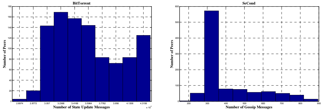
Figure 20. Histograms for (a) BitTorrent state update messages, (b) SeCond gossip messages
