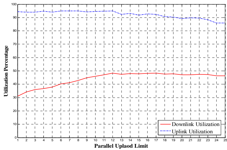
Figure 10. Parallel upload limit vs. downlink and uplink utilizations
