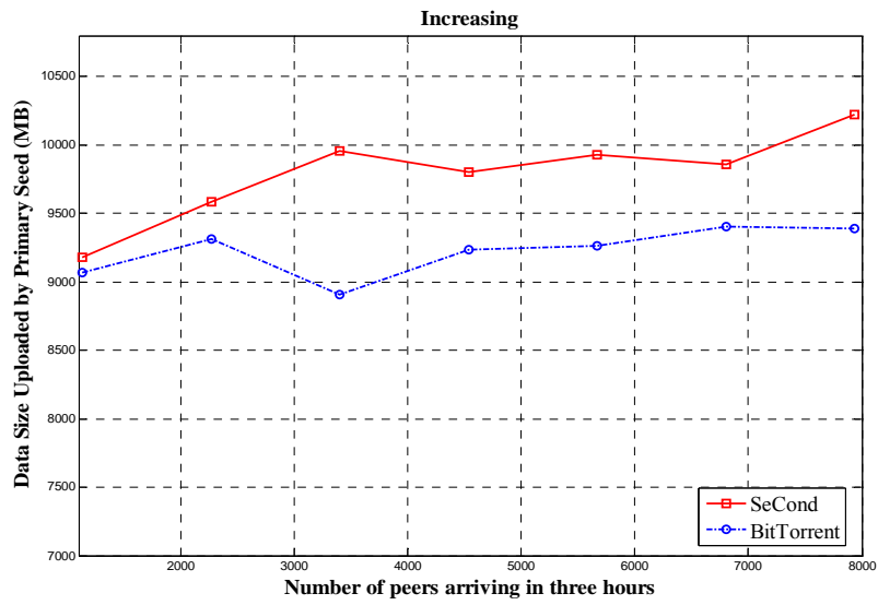
Figure 17. Load imposed on the primary seed for increasing arrival pattern vs. system size
