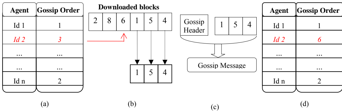
Figure 4. Gossip Message Construction example for the peer with id 2: a) Index (3) of the block that the peer with id 2 has been informed most recently is determined b) Blocks downloaded after block 6 (with index 3) are selected to be added to gossip message c) Gossip message is formed by adding header to gossip data d) Gossip order, index of the block (index 6) the destination peer is informed most recently, is updated.
