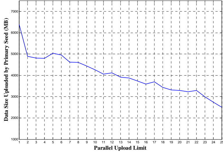
Figure 12. Parallel upload limit vs. load imposed on the primary seed
