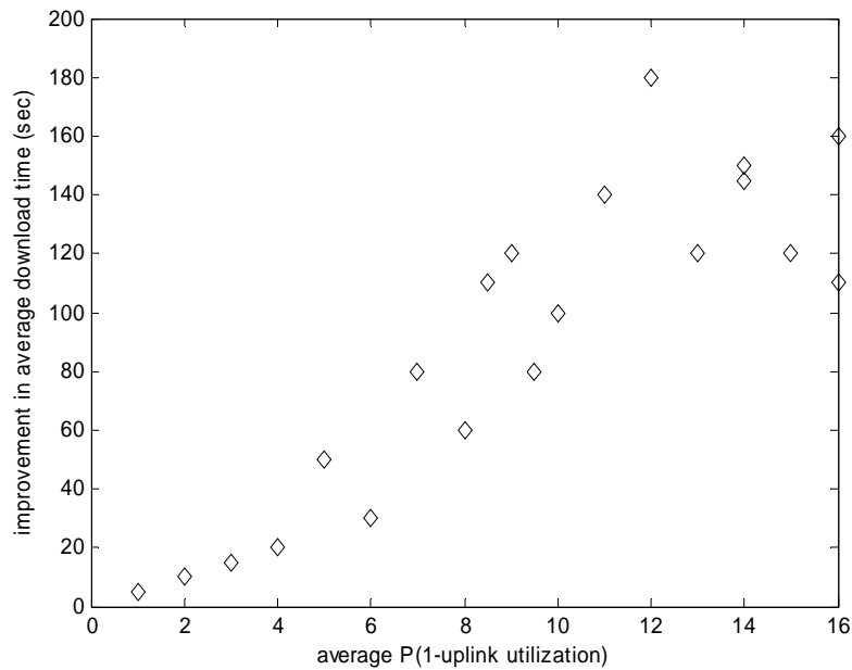
Figure 9. Improvement in average download time as a function of average P(1-uplink utilization)
