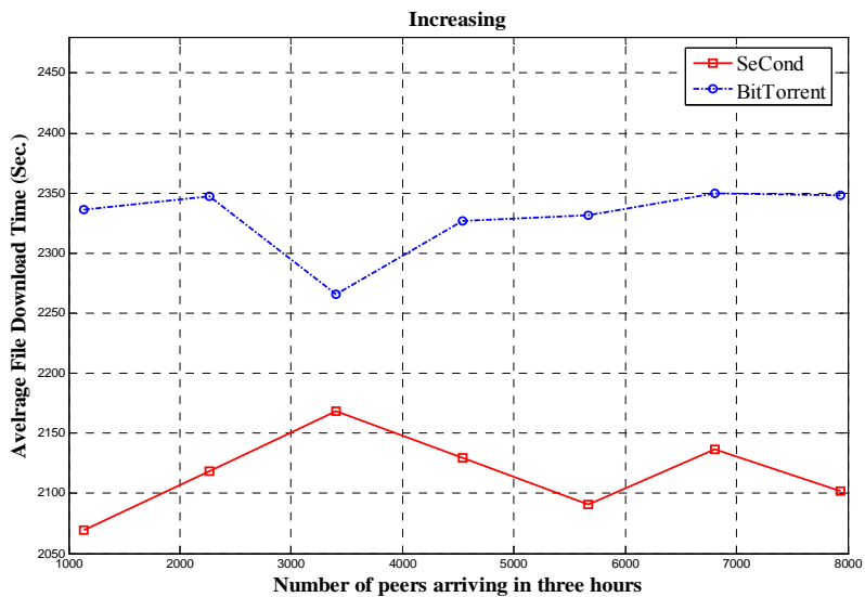
Figure 15. Average file download time for increasing arrival pattern vs. system size
