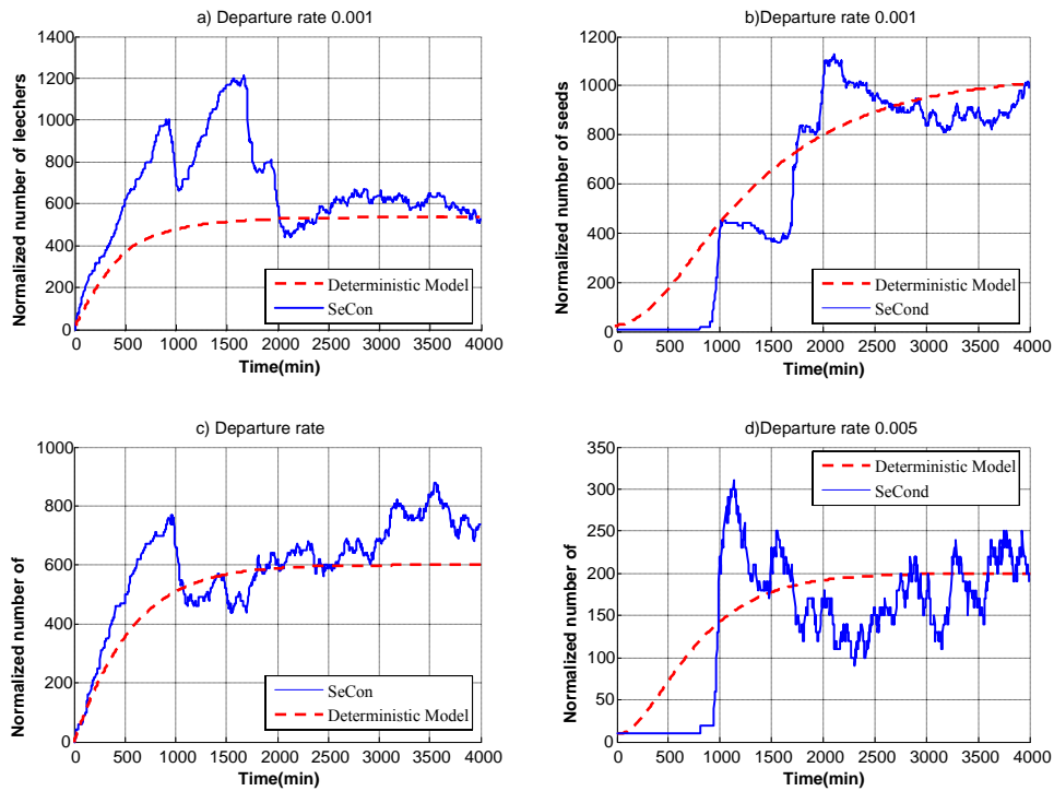
Figure 23. Deterministic model vs SeCond: Normalized number of leechers/seeds as a function of time
