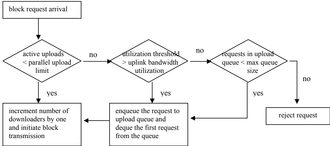
Figure 5. Illustration of upload decision process
