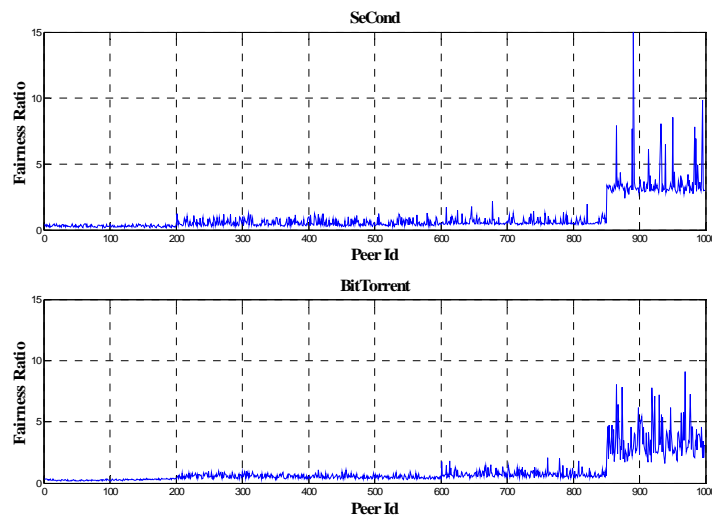
Figure 22. Fairness Ratio
