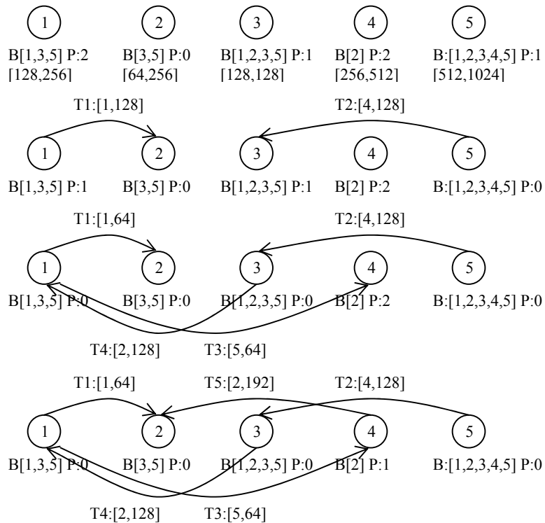
Figure 6. Illustration of block dissemination in SeCond
