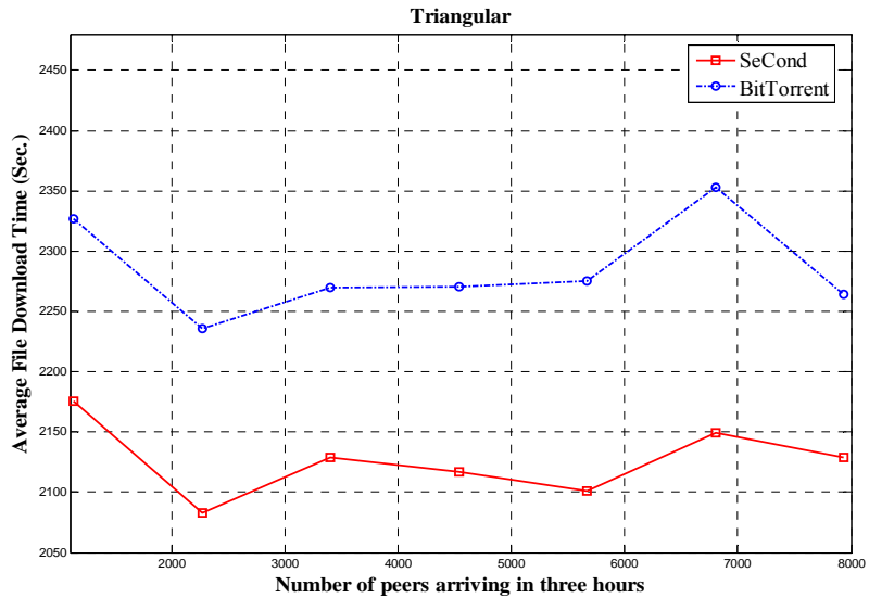
Figure 16. Average file download time for triangular arrival pattern vs. system size
