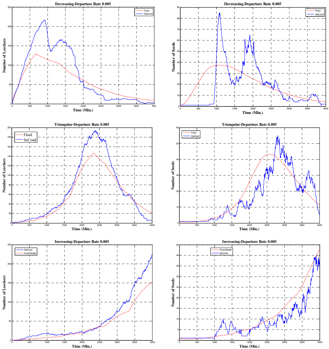
Figure 24. Deterministic model vs SeCond for (a) decreasing (b) triangular (c) increasing arrival pattern
