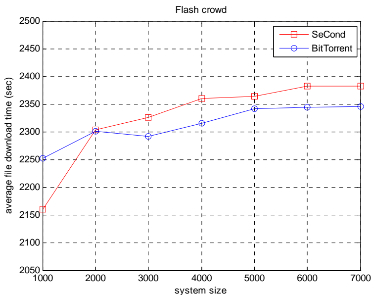
Figure 19. Flash crowd scenario: average file download time vs. system size
