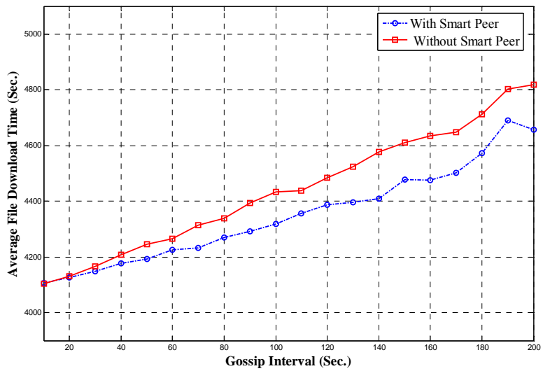
Figure 8. Effect of gossip interval on average file download time
