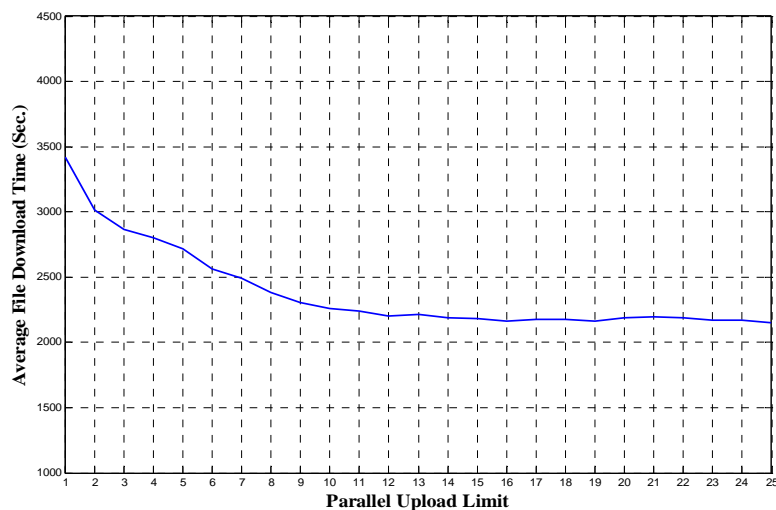
Figure 11. Effect of parallel upload limit on average file download time
