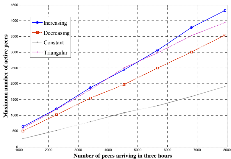
Figure 14. Maximum number of active peers vs. system size
