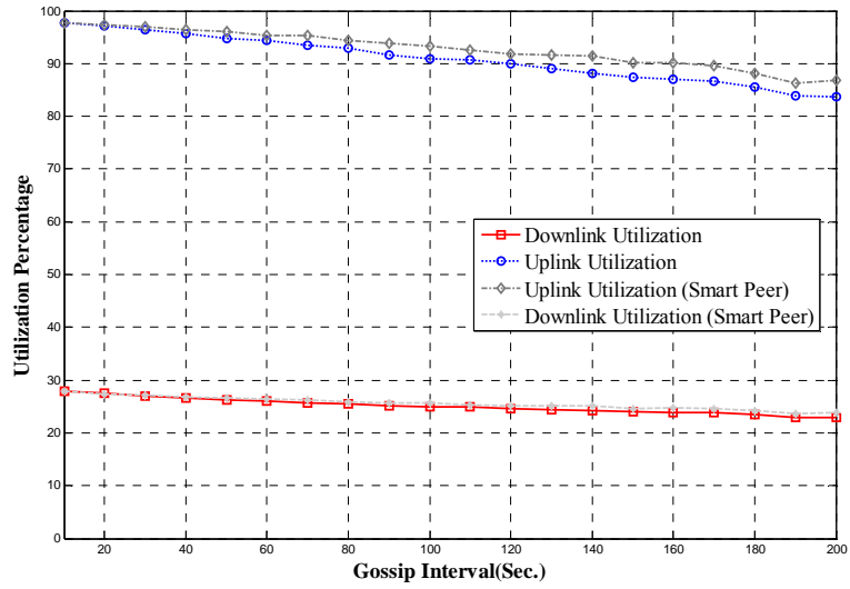
Figure 7. Effect of gossip interval on uplink/downlink utilizations
