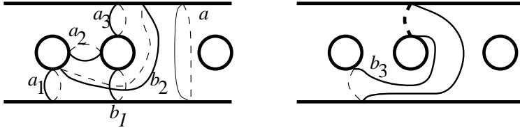
FIGURE 2. a is separating.
