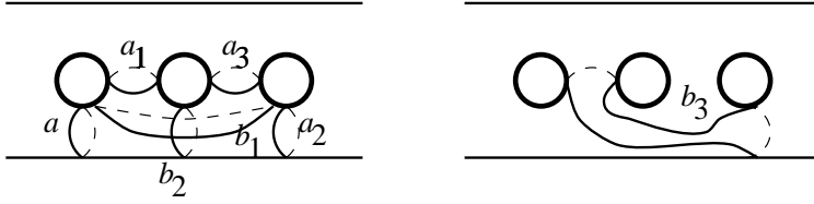
FIGURE 1. a is nonseparating.
