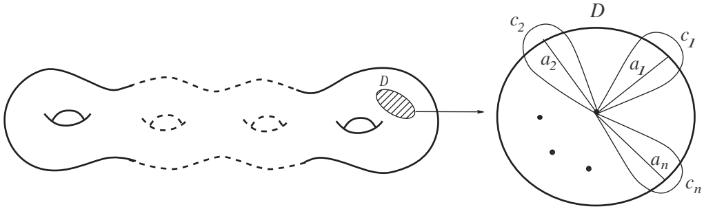
FIGURE 1. Choice for loops defining vanishing cycles.
