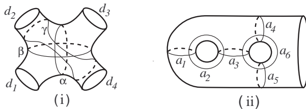
FIGURE 3. Curves of the lantern and two-holed torus relation.
