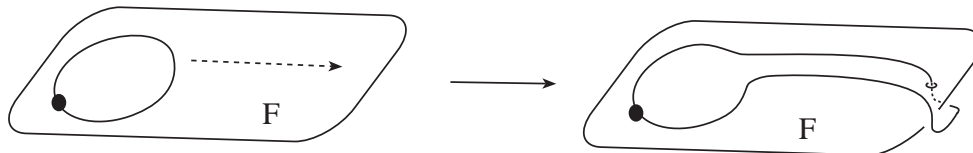
FIGURE 10. Isotopy of a dotted-circle
