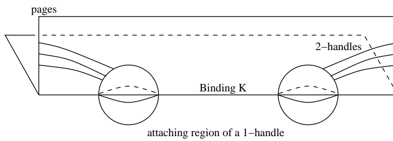
FIGURE 13. Attaching a 1-handle
