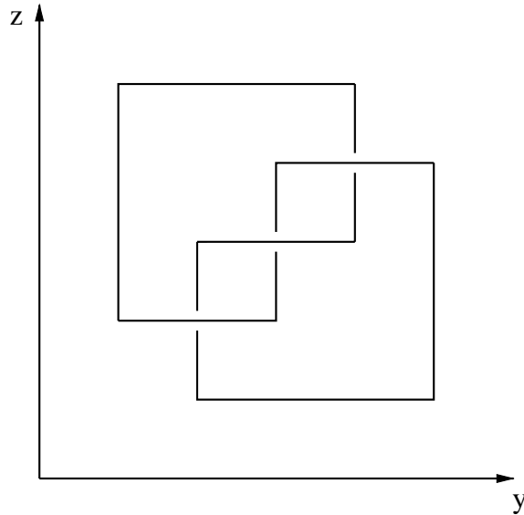
FIGURE 6. Trefoil knot in a square bridge position
