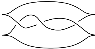
FIGURE 2. Legendrian trefoil knot
