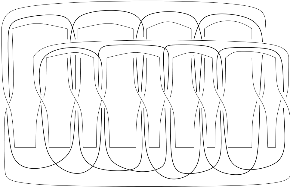
FIGURE 5. Monodromy of a (3, 5) torus knot
