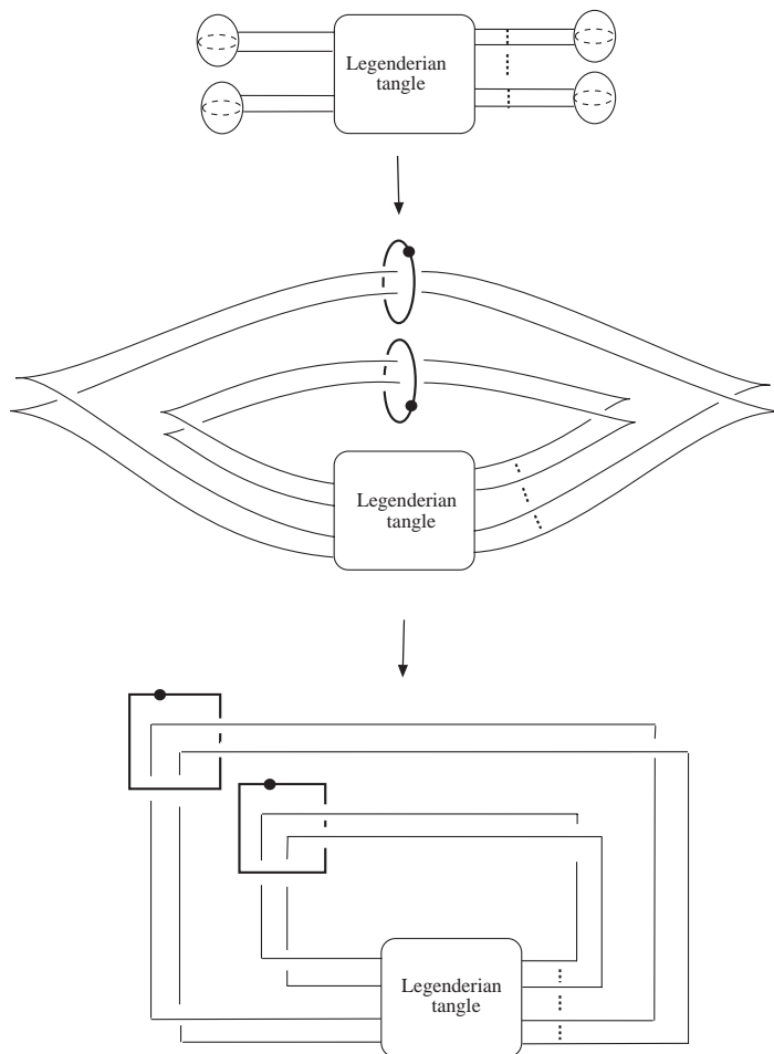
FIGURE 9. Legendrian link diagram in a square bridge position
