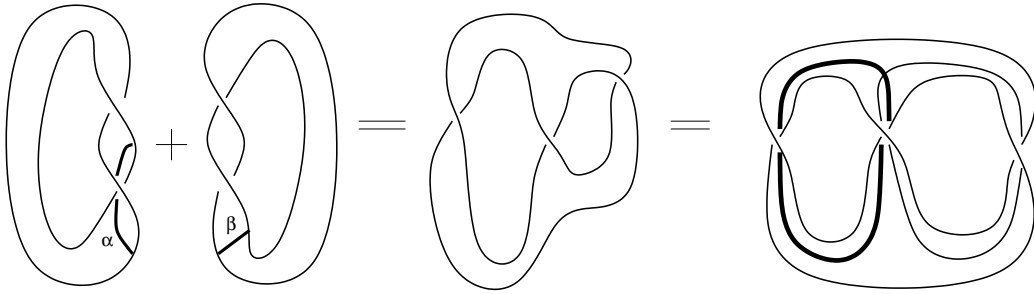
FIGURE 4. Plumbing two Hopf bands
