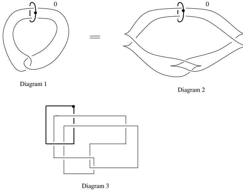
FIGURE 11. PALF on a fishtail fiber
