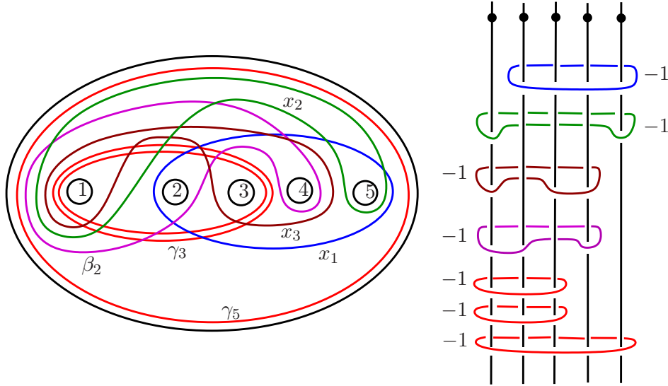
FIGURE 7. Monodromy x_1x_2x_3\beta_2\gamma_3^2\gamma_5 of the PALF on W_{(81,47)}((3, 2, 1, 3, 2)) and its handlebody diagram
