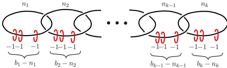
FIGURE 1. Lisca's description of the filling W_{(p,q)}(\mathbf{n})
