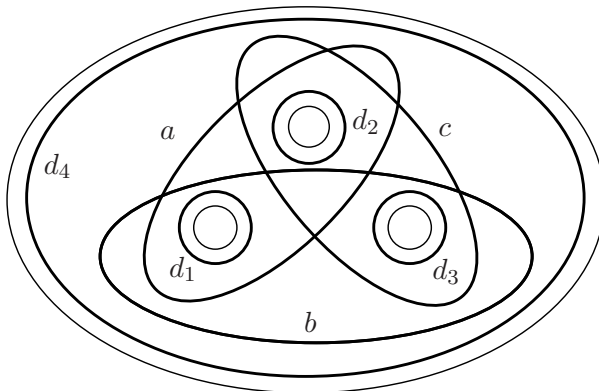
FIGURE 8. The lantern relation d_1d_2d_3d_4 = abc on a four-holed sphere
