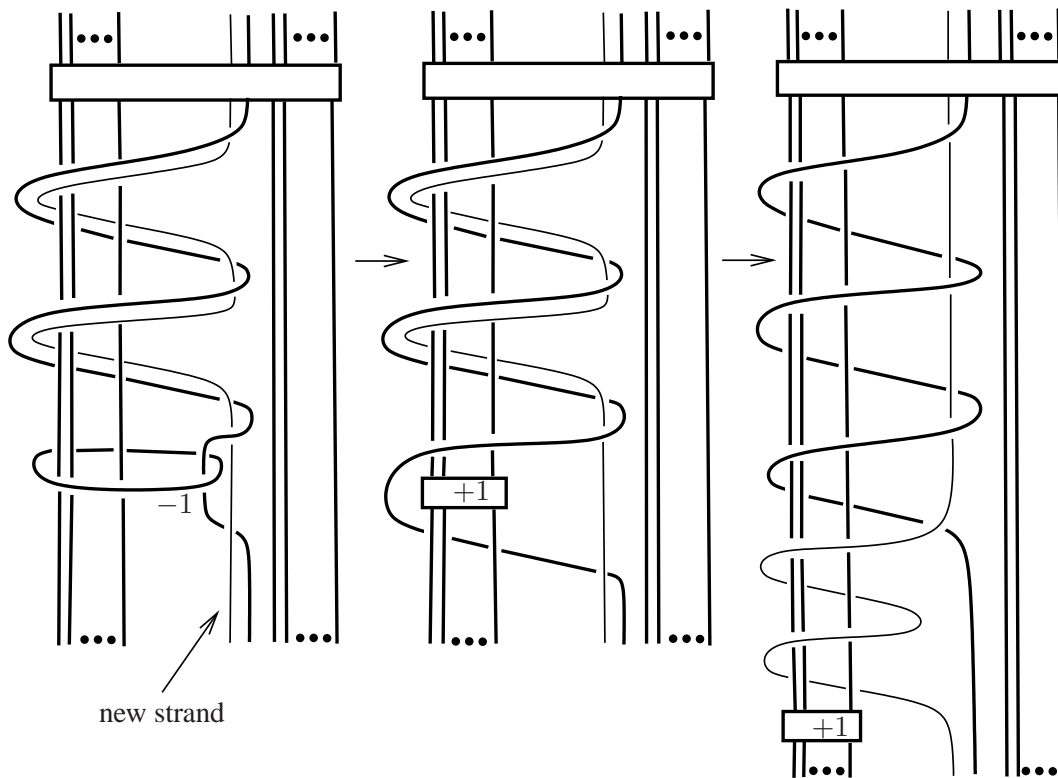
FIGURE 4. Blowing down the (-1) -curve
