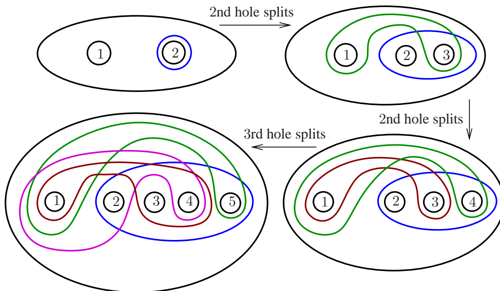
FIGURE 6. Positive stabilizations of the standard open book of S^1 \times S^2
