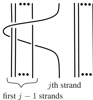
FIGURE 2. The j th strand wraps around the first j - 1 strands once
