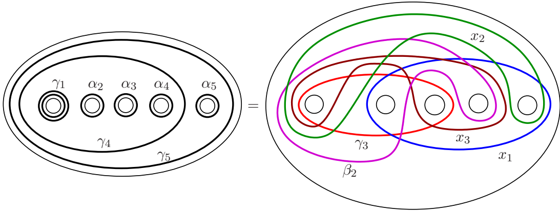
FIGURE 10. A monodromy substitution: \alpha_2\alpha_3\alpha_4\alpha_5\gamma_1^2\gamma_4\gamma_5 = x_1x_2x_3\beta_2\gamma_3 .
