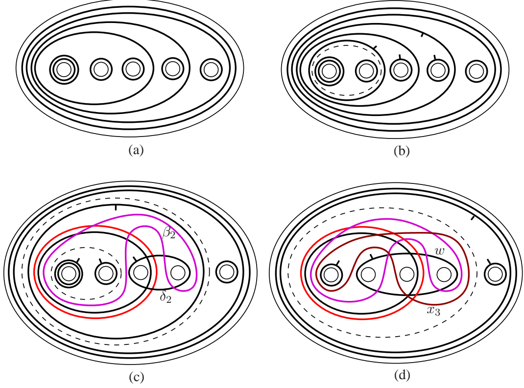
FIGURE 9. Thicker curves indicate right-handed Dehn twists on a 5-holed disk, where left-handed Dehn twists are drawn as dashed curves
